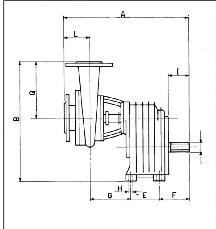
VALORI INDICATIVI POMPE CARRELLATE SERIE PM/T - OVERALL DIMENSIONS FOR PM/T SERIES PUMPS DIMENSIONS D'ENCOMBREMENT ET POIDS
